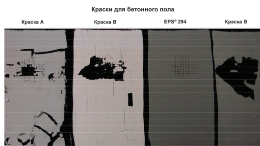
FIGURE 11. EPS® 294 COMPARED TO COMPETITIVE PAINTS AFTER 2 HOUR WATER IMMERSION AND CROSSCUT/TAPE ADHESION TEST
